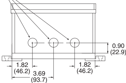
Optional Mounting Bracket (MB)
