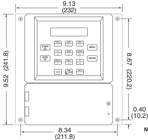
Optional Mounting Bracket (MB)
